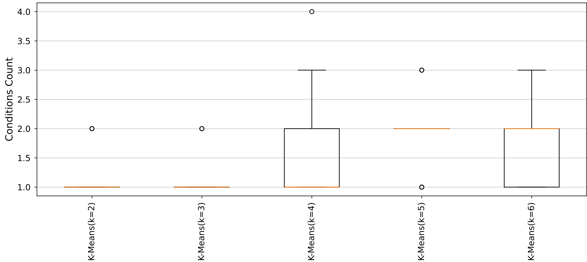
YARA Rules Conditions Count Distribution (Cluster28_Size6 dataset)
